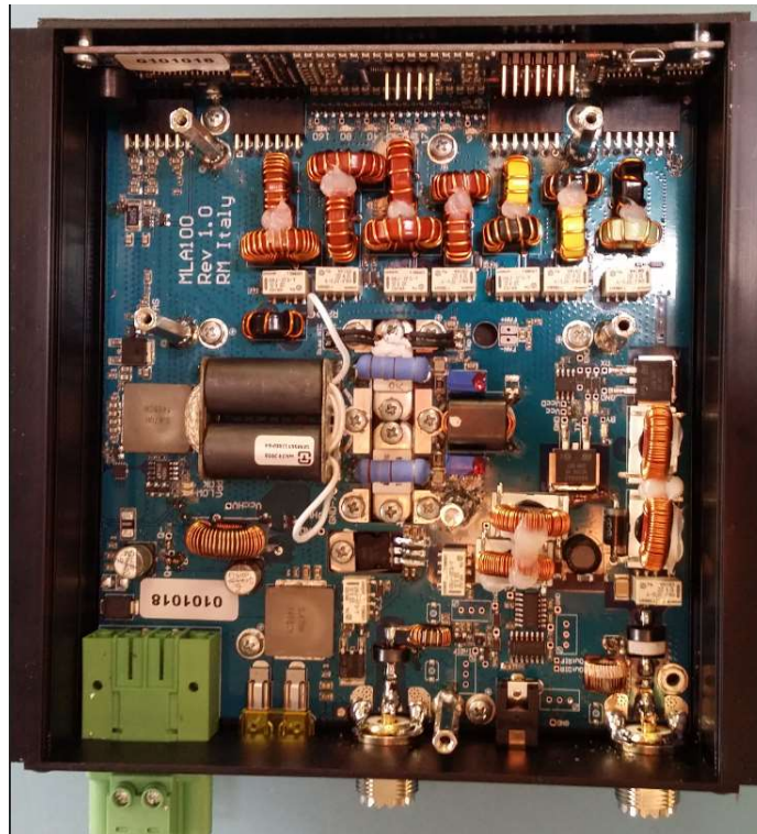
View of top side of main board of MLA 100 Power Amplifier
