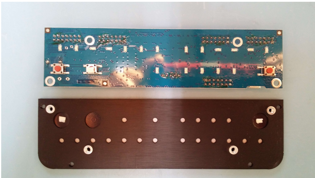
View of bottom side of control and indicator board of MLA 100 Power Amplifier
