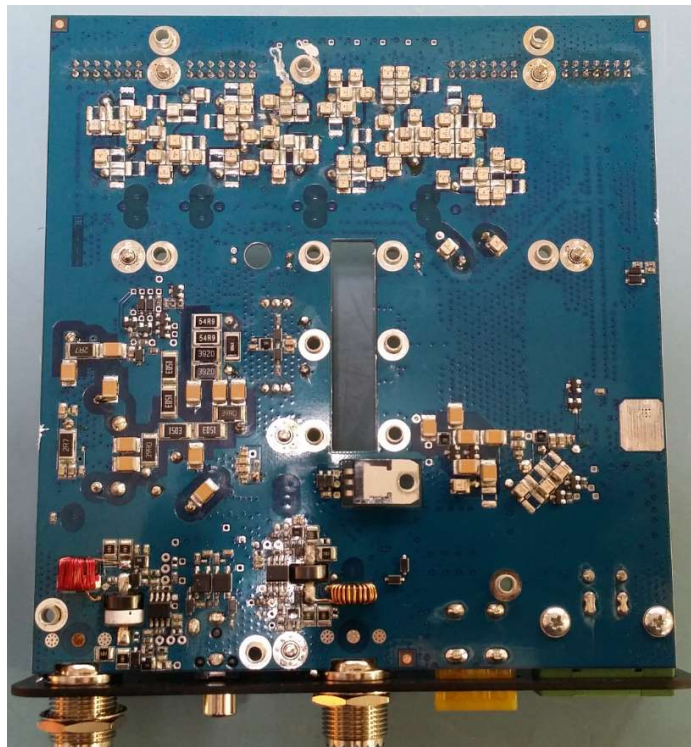
View of bottom side of main board of MLA 100 Power Amplifier
