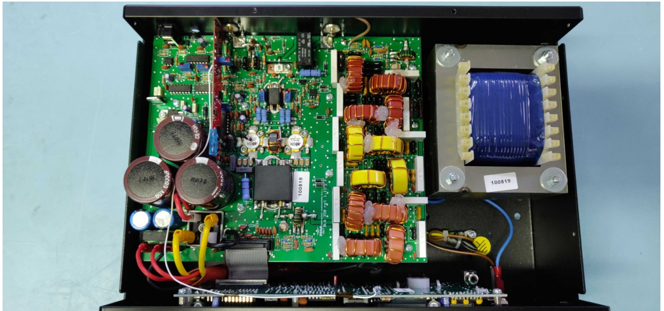
1. Top view - Main PCB
