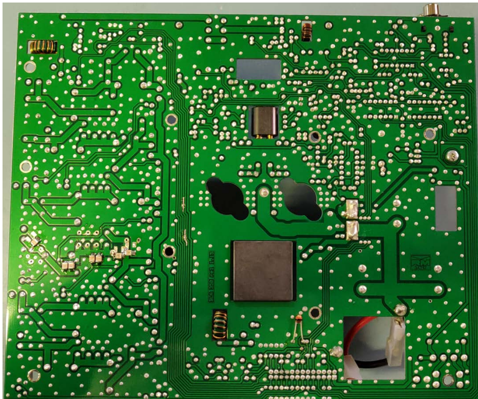
2. Bottom view - Main PCB
