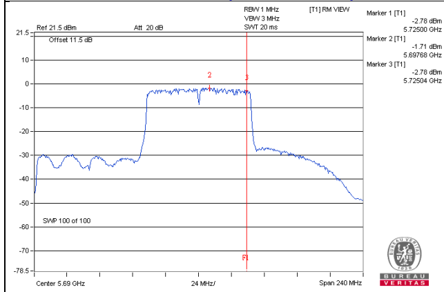
802.11ac (VHT80+80) / Chain 3 CH138(UNII-2C Band)
