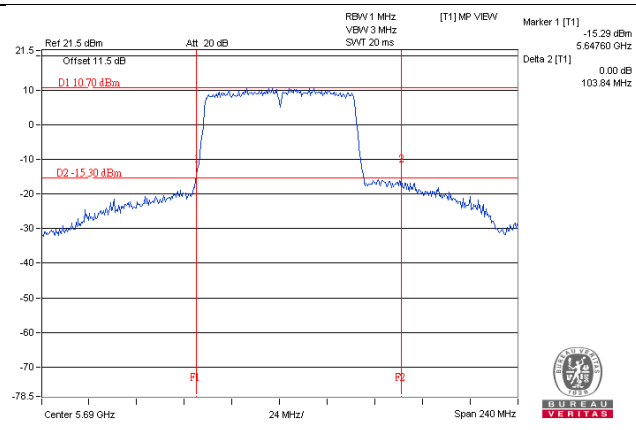
802.11ac (VHT80+80) / Chain 1 - CH138 (UNII-2C Band)
