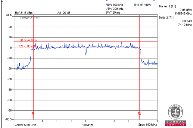
802.11ac (VHT80+80) / Chain 0 - CH138 (UNII-3 Band)
