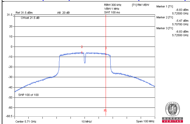
802.11ac (VHT80+80) / Chain 0– CH138(UNII-3 Band)
