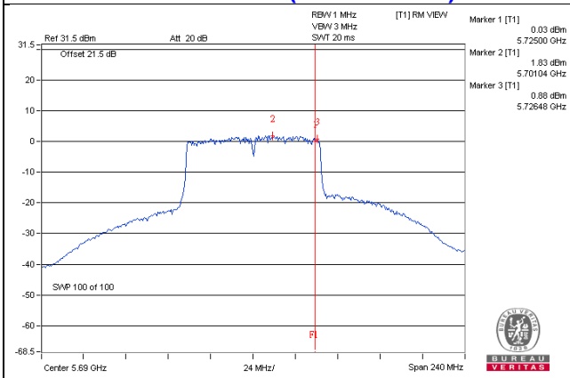
802.11ac (VHT80+80) / Chain 0 CH138(UNII-2C Band)
