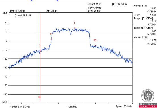
802.11ac(VHT40) / CH151
