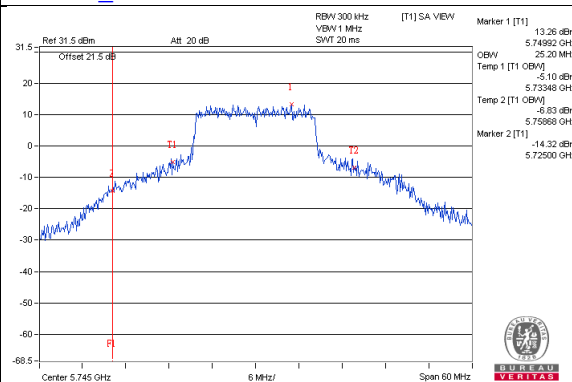
802.11ac(VHT20)_Chain1 / CH149
