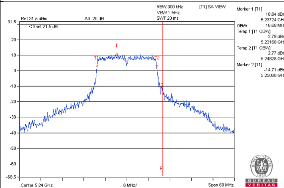
802.11ac(VHT20)_Chain0 / CH48
