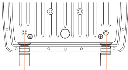
Connect a ground cable from the outdoor unit to an appropriate grounding point.
