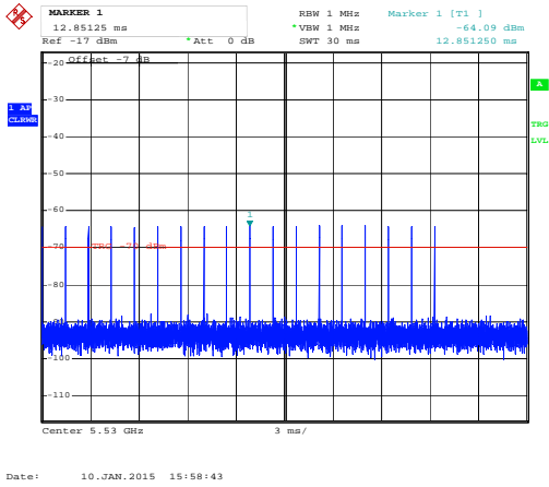
Radar #2 DFS detection threshold level
