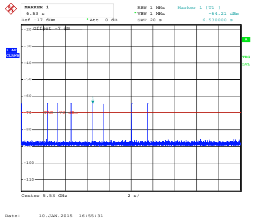
Radar #6 DFS detection threshold level
