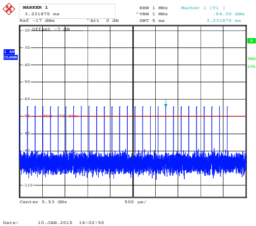
Radar #3 DFS detection threshold level
