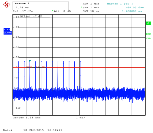
Radar #5 DFS detection threshold level
