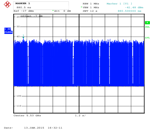
Master (EUT) Data Traffic Plot
