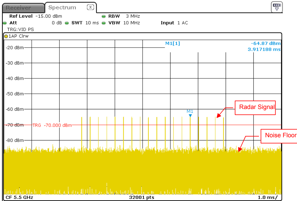
Radar Signal 3
