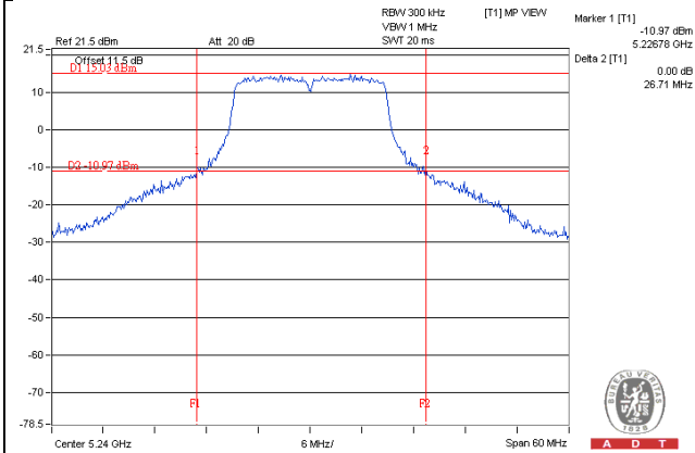
802.11ac (VHT20)_3TX
