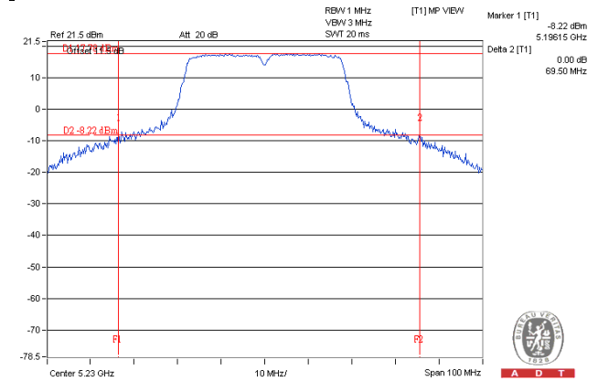
802.11ac (VHT40)_3TX
