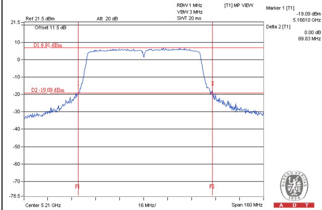
802.11ac (VHT80)_3TX
