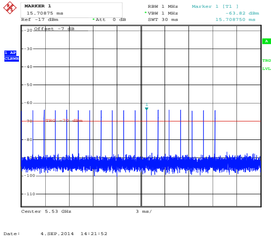
Radar #2 DFS detection threshold level
