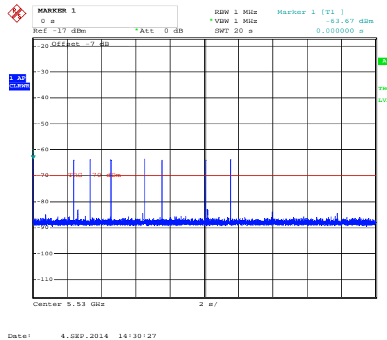
Radar #6 DFS detection threshold level
