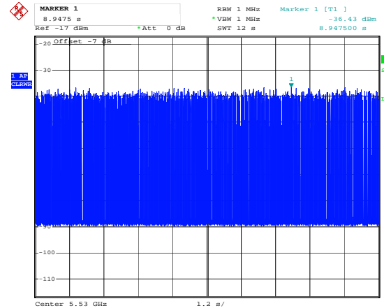
Master (EUT) Data Traffic Plot
