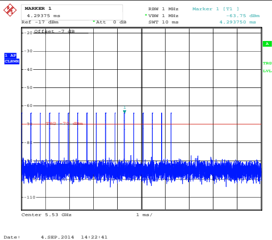
Radar #3 DFS detection threshold level
