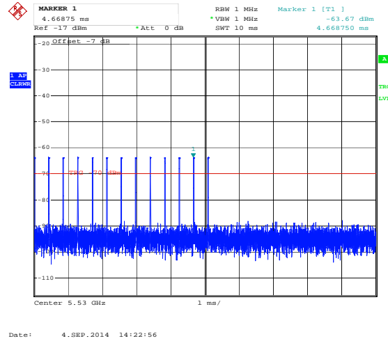
Radar #5 DFS detection threshold level
