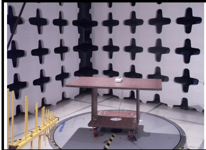
Test Setup Photo -5 (Internal Antenna)
