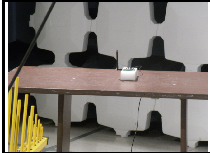
Test Setup Photo -3 (Ext Antenna)
