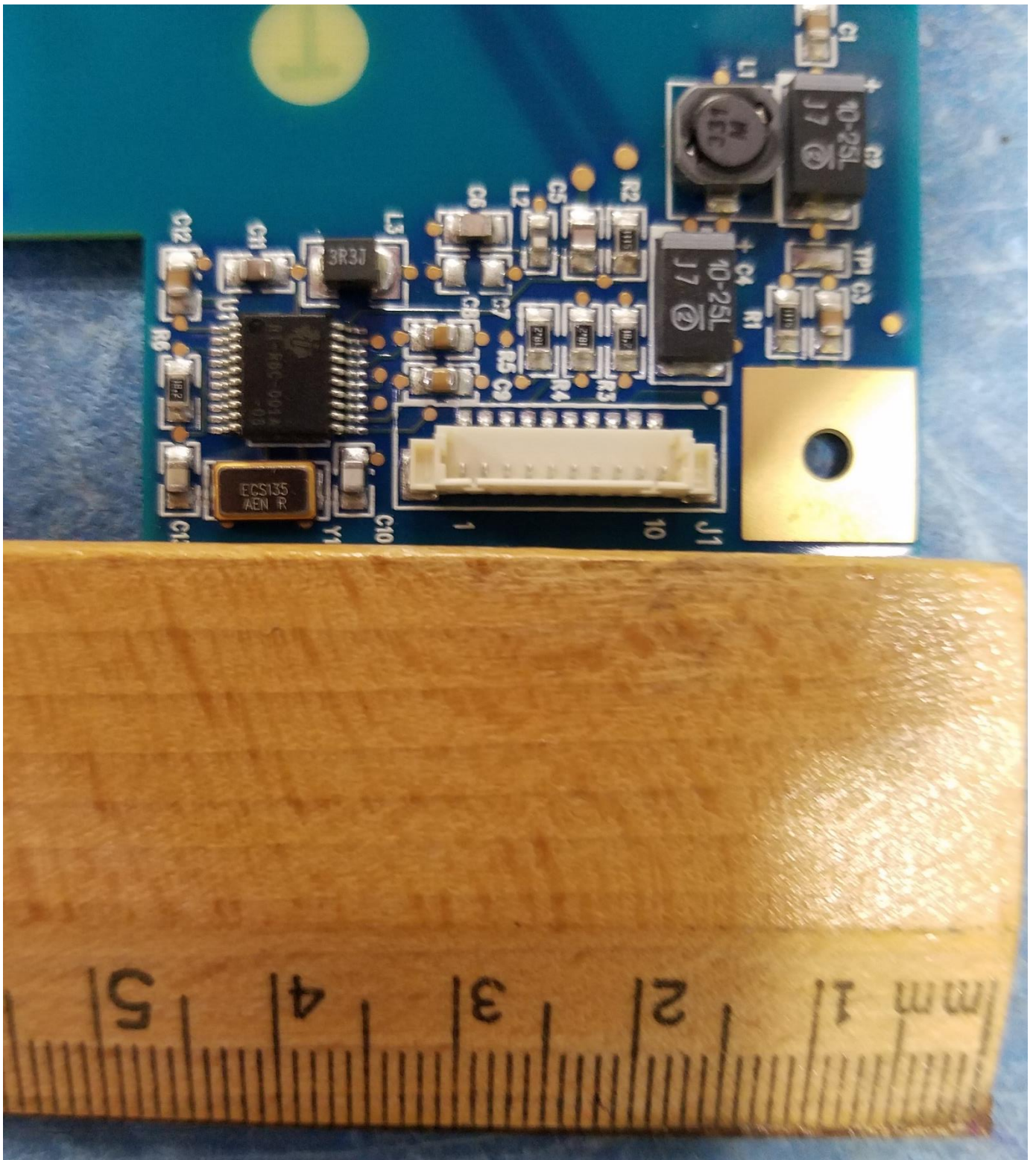
Figure 2: RFID Circuit Top View- Showing Component Markings
