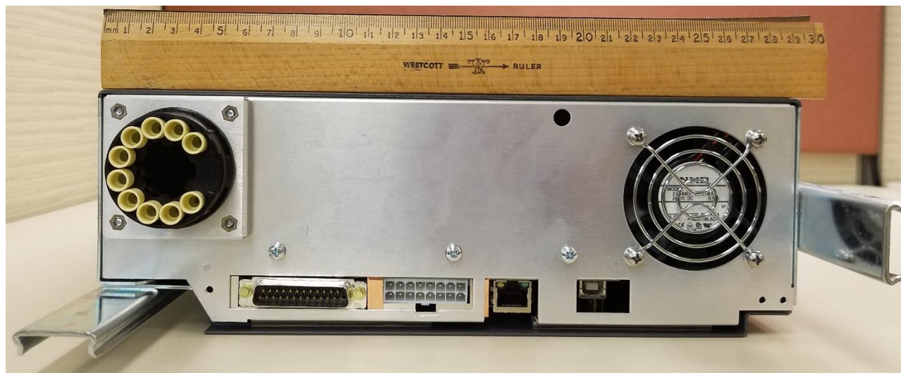
Figure 6: Chemcassette® Analyzer Side Four
