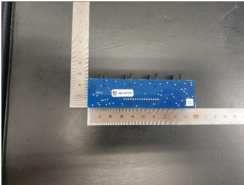
Tranceducer Board_1 rear side
