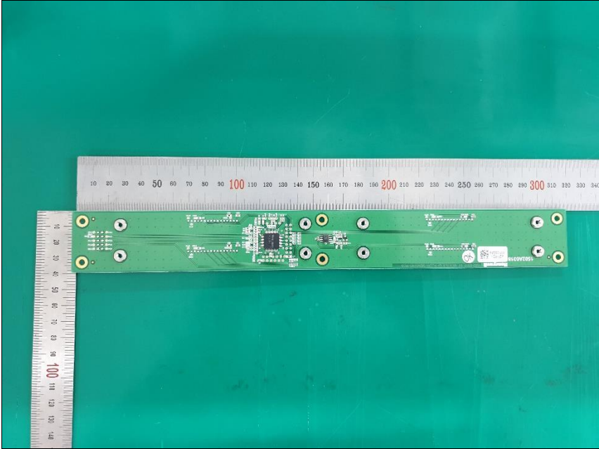
Flow Sensing Board rear side
