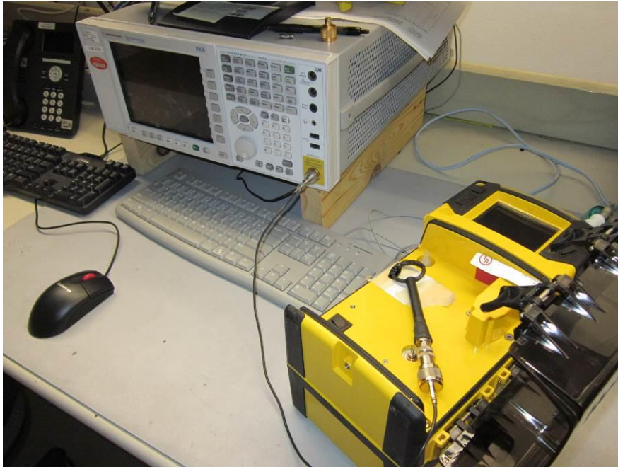
Figure 9 Test Setup for Occupied Bandwidth
