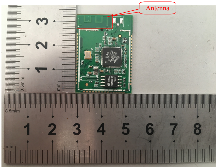
EUT – Shielding off View
