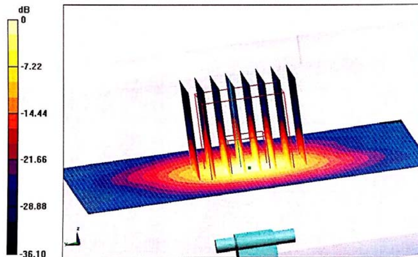
0 dB = 17.6 W/kg = 12.46 dBW/kg
