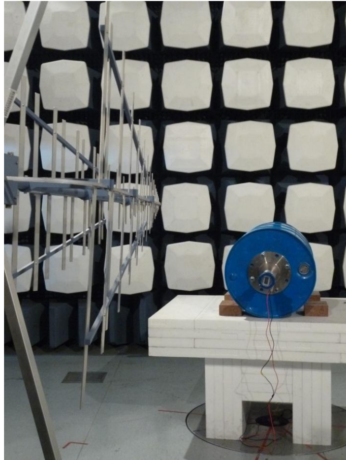
Photograph 1: Set-up for Radiated Spurious Emissions, below 1GHz
