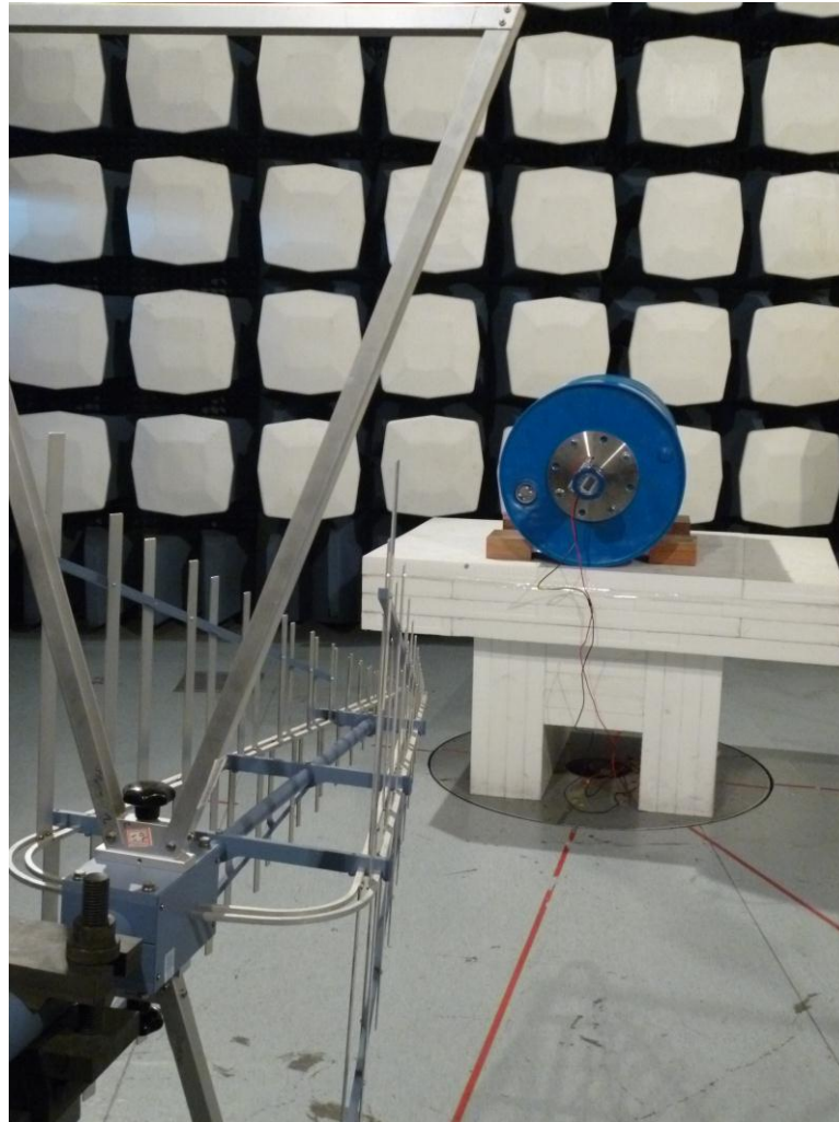
Photograph 1: Set-up for Radiated Spurious Emissions, below 1GHz
