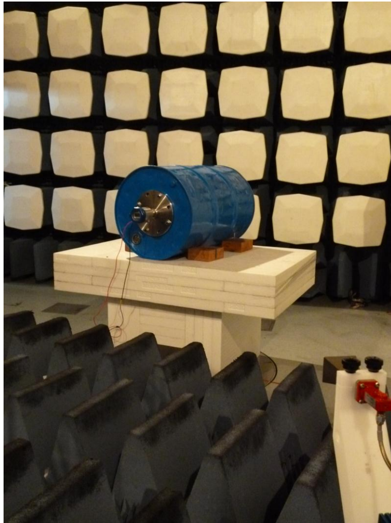
18-26.5GHz
