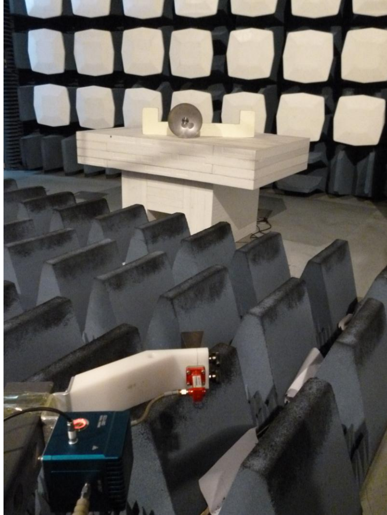
Photograph 4: Set-up for Fundamental emission test
