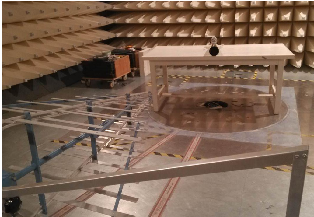
Photograph 2: Set-up for Spurious Emissions, above 1GHz
