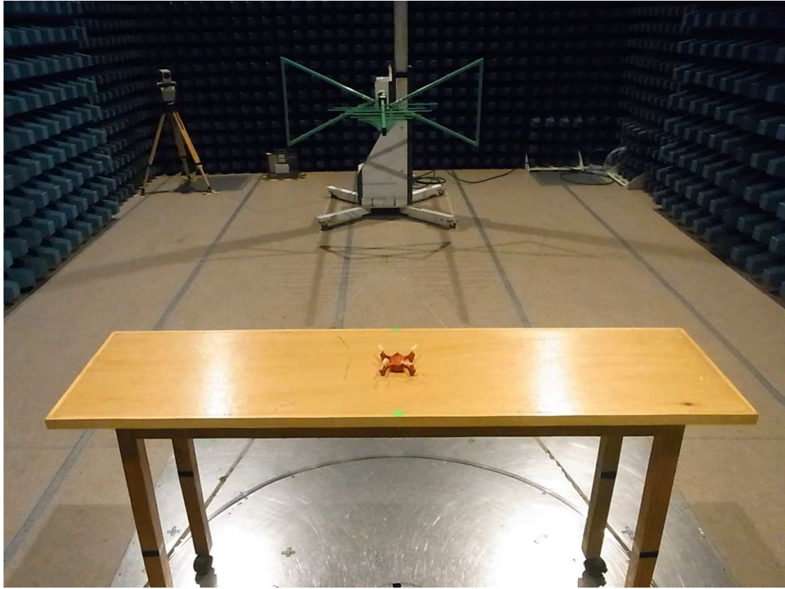
Front view (30MHz – 1GHz)
