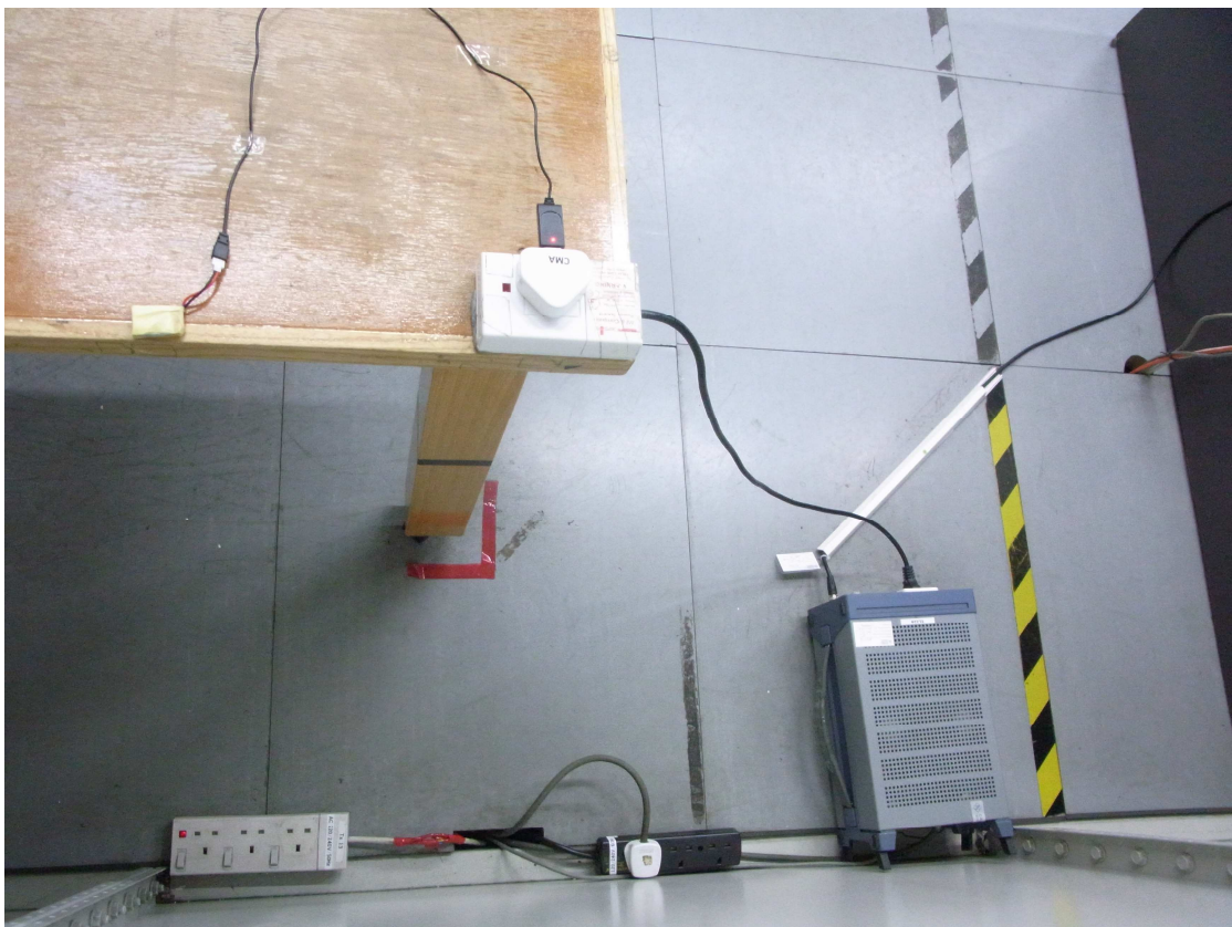
Conducted emission (Back view)
