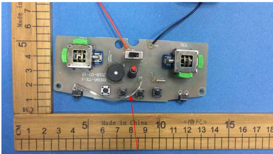
Wire Antenna
