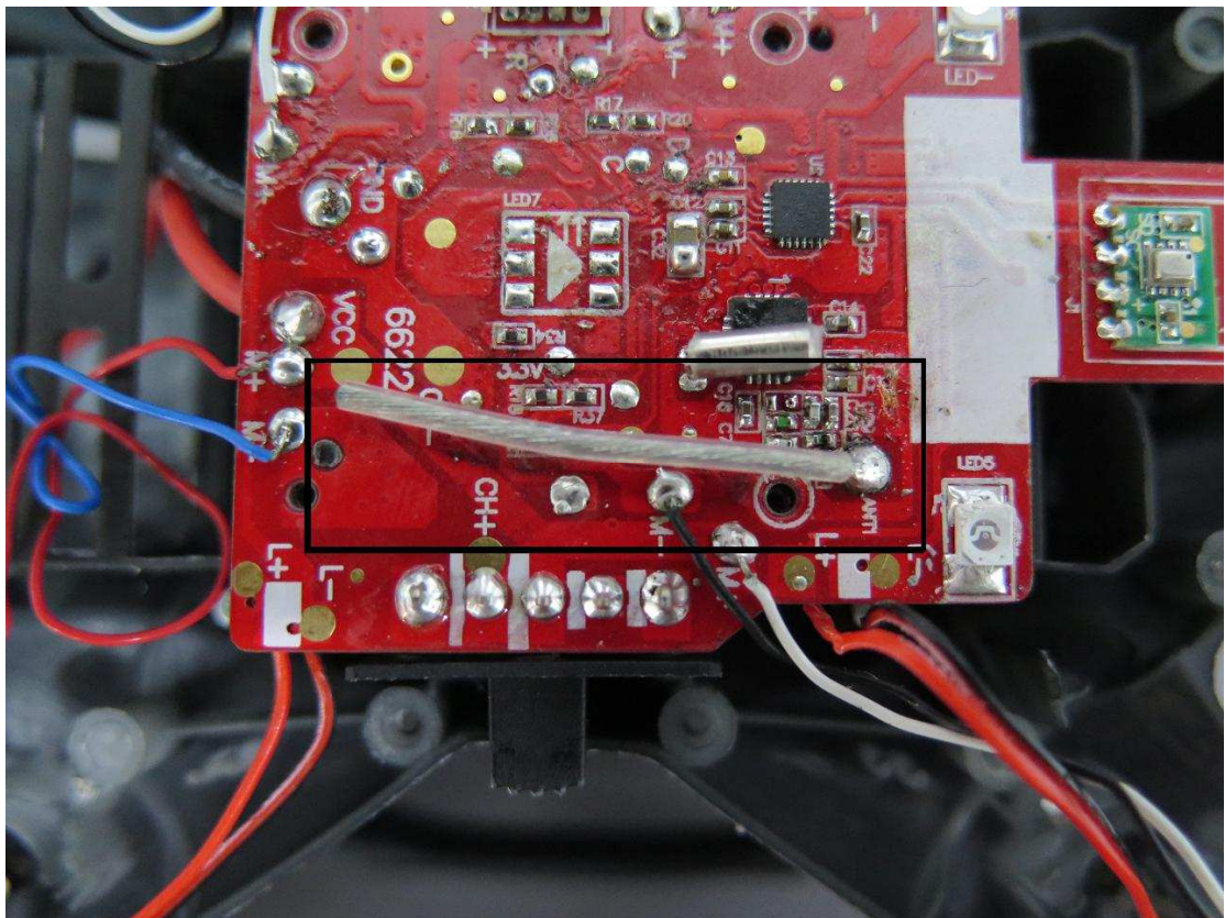
EUT antenna 1 (Self-develop RF module)
