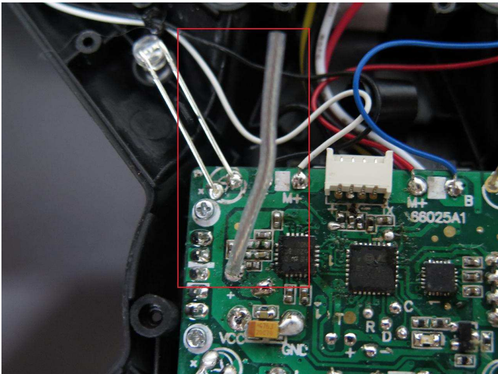
EUT antenna 1 (Self-develop RF module)
