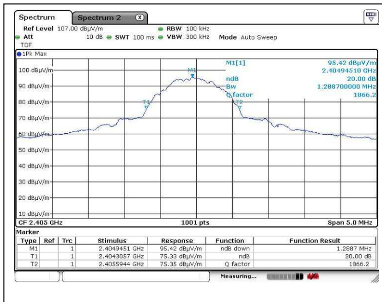
Bandwidth 1 (2405MHz)
