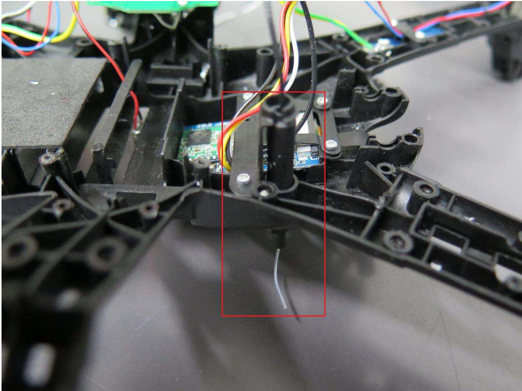
EUT antenna 2 (WiFi)
