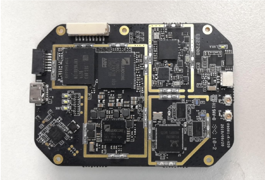
FRONT VIEW OF EUT (WITHOUT SHIELDING)
