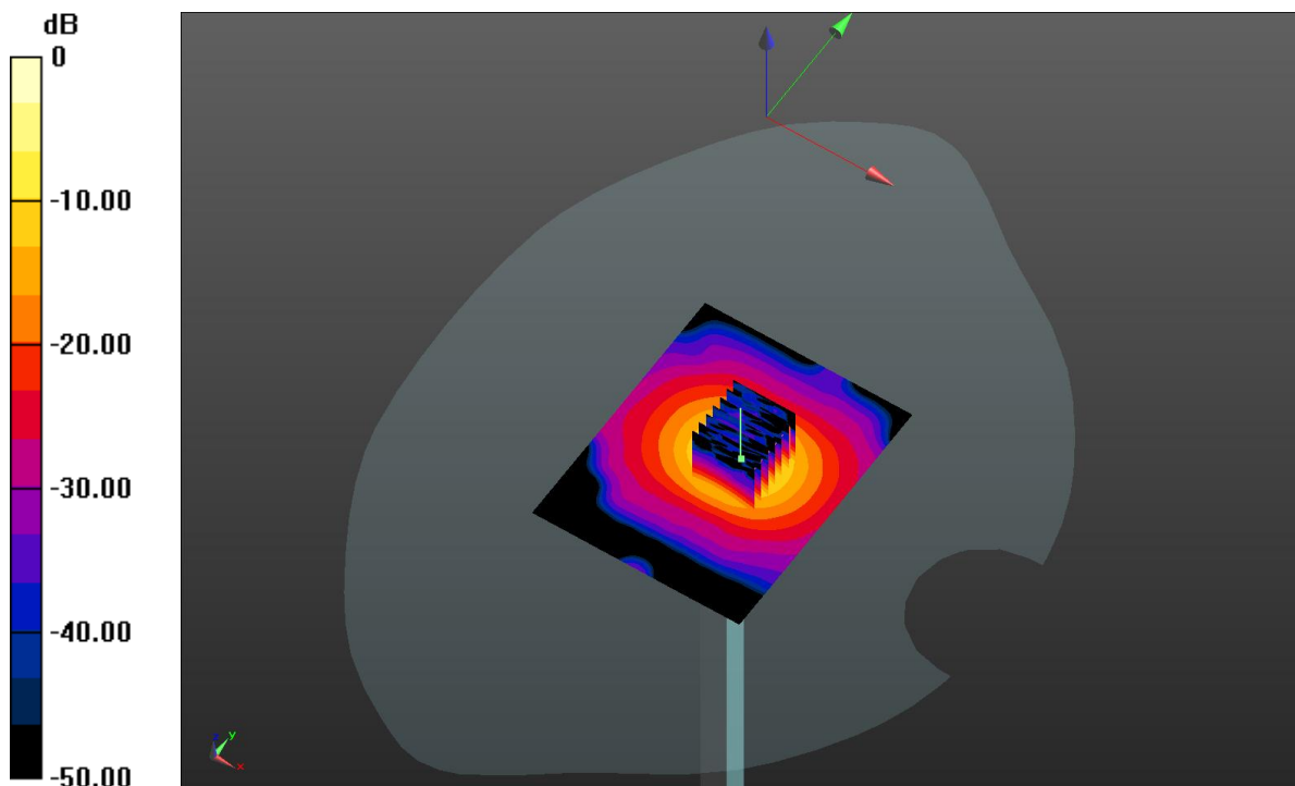
0 dB = 17.1 W/kg
