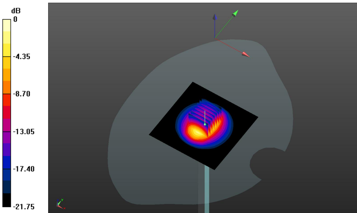
0 dB = 6.05 W/kg
