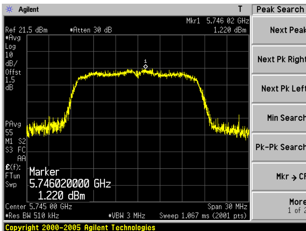
Channel 149 (5745MHz)
