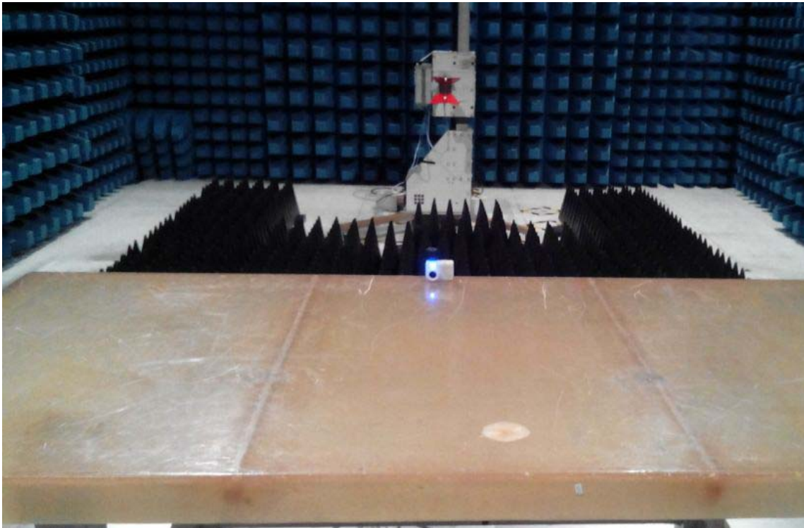
Description: Radiated Emission Test Setup for 1~18GHz
