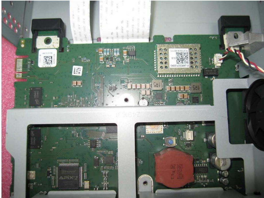
BE L003 internal photos. FCC ID 2ACRLBEL005
