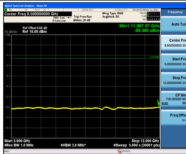
Band5-1.4MHz-QPSK-20525-1-0-Low-5000-12000--59.36-PASS
