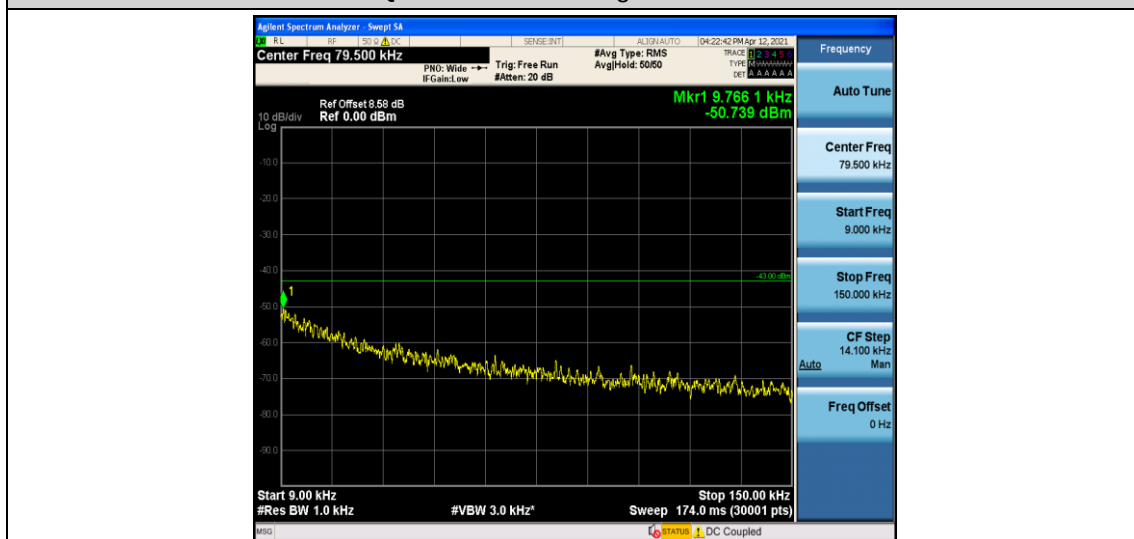
Band5-1.4MHz-16QAM-20407-1-0-Low-0.009-0.15--50.74-PASS
