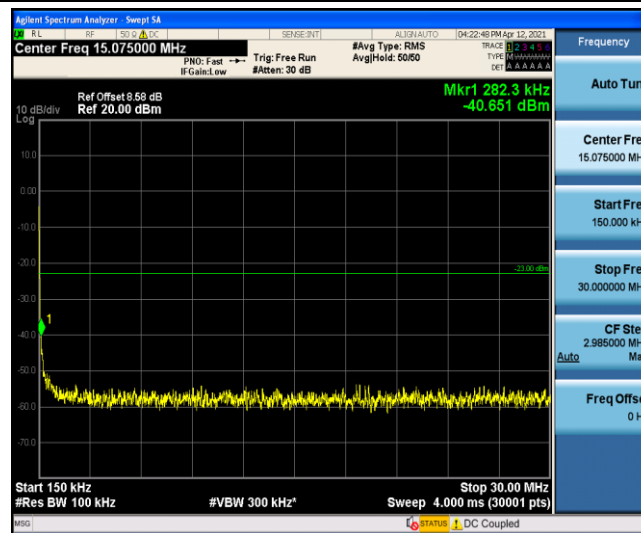
Band5-1.4MHz-16QAM-20407-1-0-Low-0.15-30--40.65-PASS
