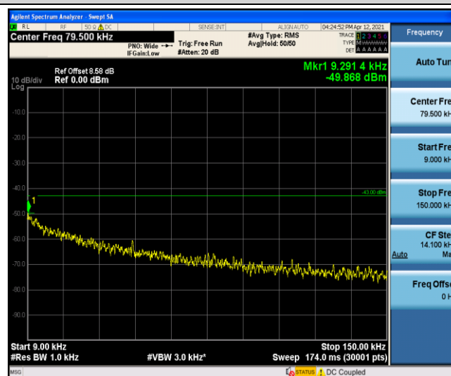
Band5-1.4MHz-QPSK-20525-1-0-Low-0.009-0.15--49.87-PASS
