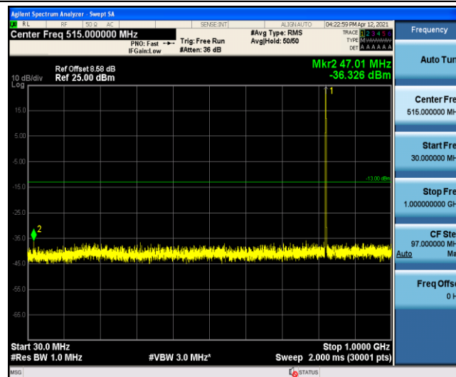
Band5-1.4MHz-16QAM-20407-1-0-Low-30-1000--36.33-PASS
