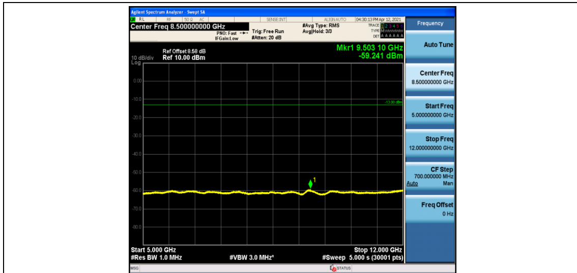
Band5-1.4MHz-QPSK-20643-1-0-High-5000-12000--59.24-PASS
