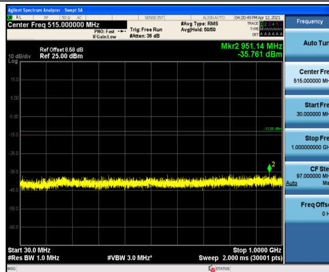
Band5-1.4MHz-QPSK-20407-1-0-Low-30-1000--35.76-PASS
