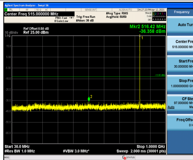
Band5-1.4MHz-16QAM-20525-1-0-Low-30-1000--36.36-PASS
