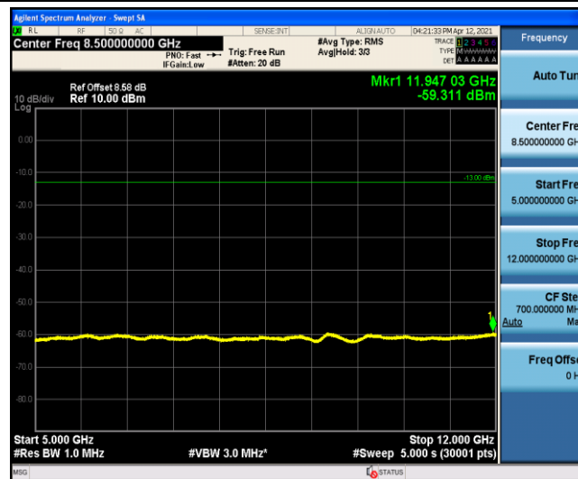
Band5-1.4MHz-QPSK-20407-1-0-Low-5000-12000--59.31-PASS
