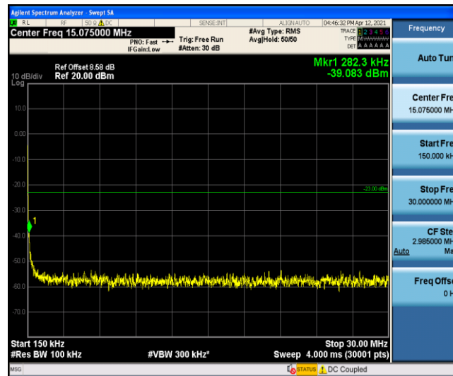
Band5-3MHz-QPSK-20415-1-0-Low-0.15-30--39.08-PASS
