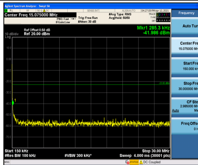
Band5-1.4MHz-16QAM-20525-1-0-Low-0.15-30--41.99-PASS
