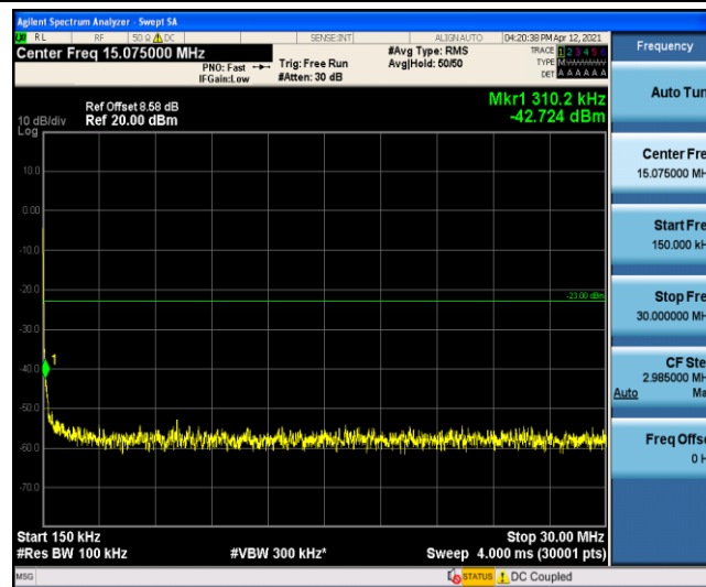
Band5-1.4MHz-QPSK-20407-1-0-Low-0.15-30--42.72-PASS
