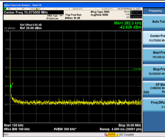
Band5-1.4MHz-QPSK-20525-1-0-Low-0.15-30--42.63-PASS
