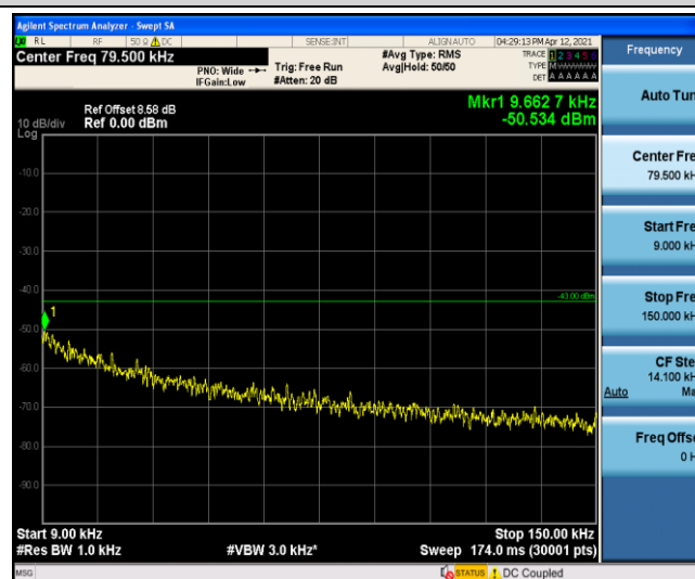
Band5-1.4MHz-QPSK-20643-1-0-High-0.009-0.15--50.53-PASS
