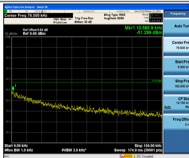
Band5-1.4MHz-16QAM-20525-1-0-Low-0.009-0.15--51.3-PASS
