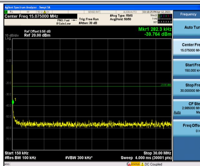
Band4-20MHz-QPSK-20050-1-0-Low-0.15-30
