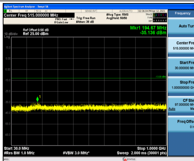
Band4-15MHz-QPSK-20175-1-0-Low-30-1000
