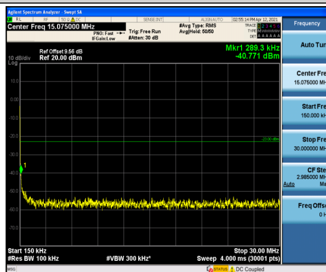
Band4-15MHz-16QAM-20025-1-0-Low-0.15-30
