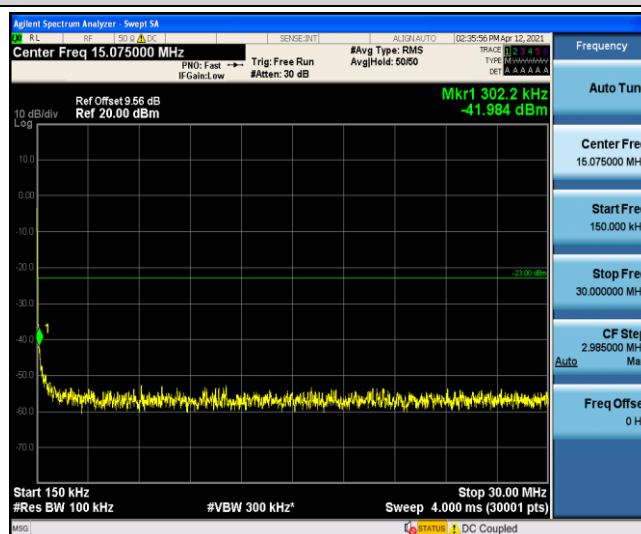
Band4-15MHz-QPSK-20175-1-0-Low-0.15-30
