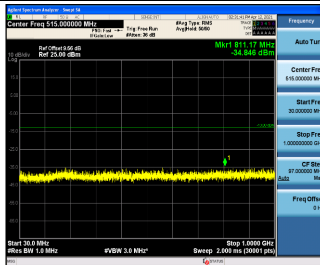
Band4-15MHz-QPSK-20325-1-0-High-30-1000
