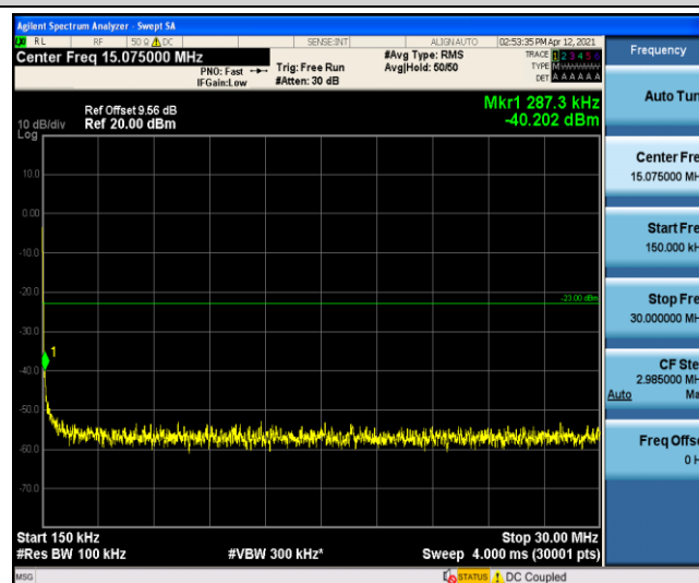
Band4-15MHz-QPSK-20025-1-0-Low-0.15-30
