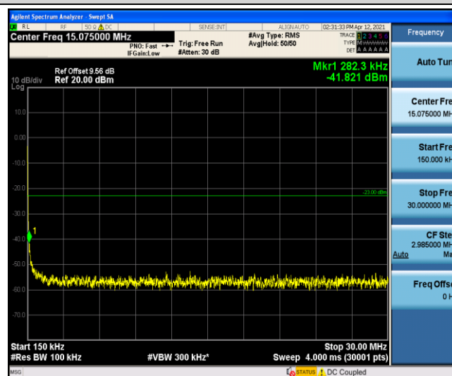
Band4-15MHz-QPSK-20325-1-0-High-0.15-30
