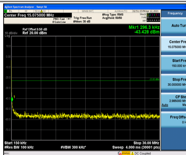
Band4-10MHz-16QAM-20350-1-0-High-0.15-30
