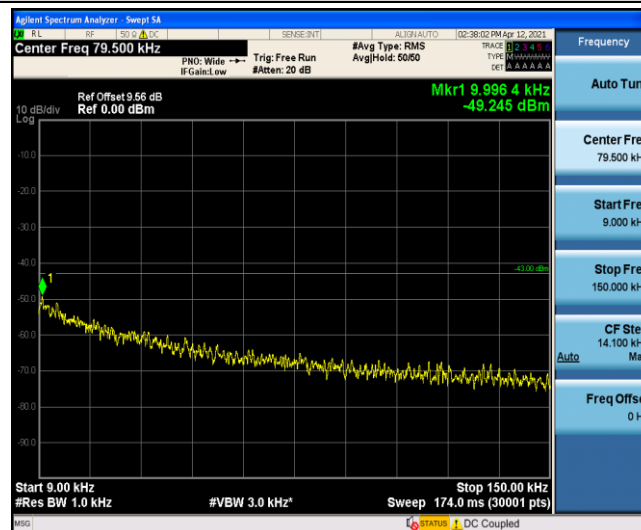
Band4-15MHz-16QAM-20175-1-0-Low-0.009-0.15
