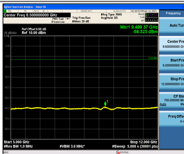
Band4-15MHz-QPSK-20175-1-0-Low-5000-12000
