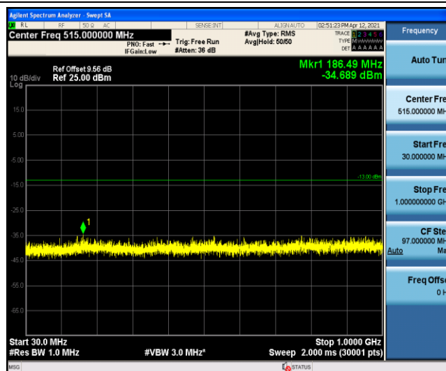
Band4-10MHz-16QAM-20350-1-0-High-30-1000
