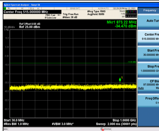
Band4-10MHz-16QAM-20175-1-0-Low-30-1000
