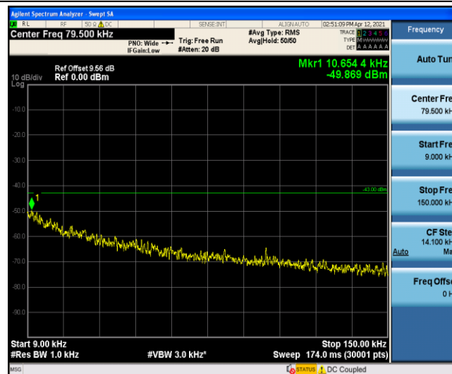
Band4-10MHz-16QAM-20350-1-0-High-0.009-0.15
