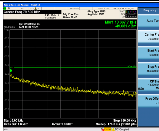
Band4-20MHz-QPSK-20050-1-0-Low-0.009-0.15
