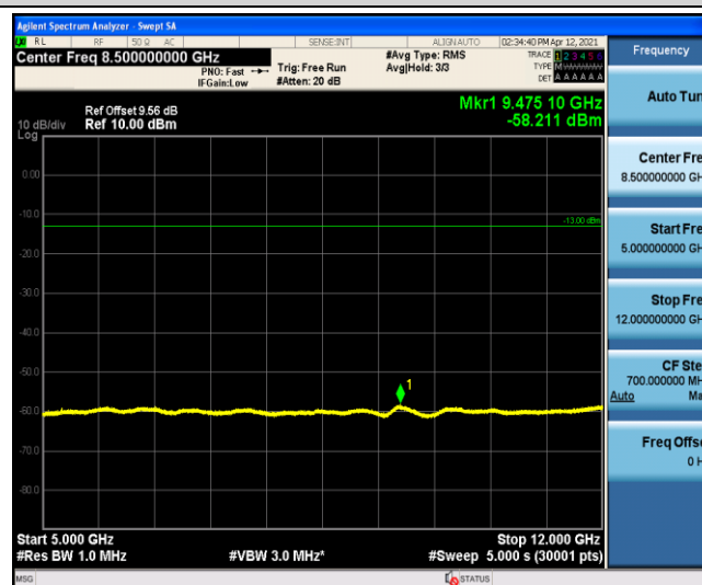
Band4-15MHz-16QAM-20325-1-0-High-5000-12000
