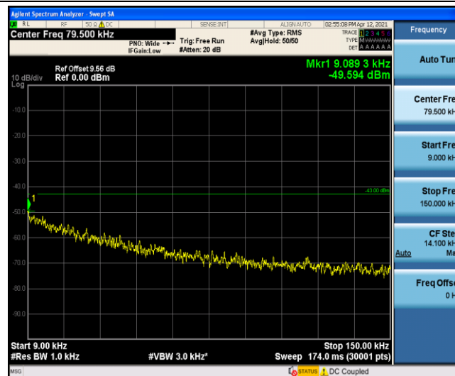
Band4-15MHz-16QAM-20025-1-0-Low-0.009-0.15
