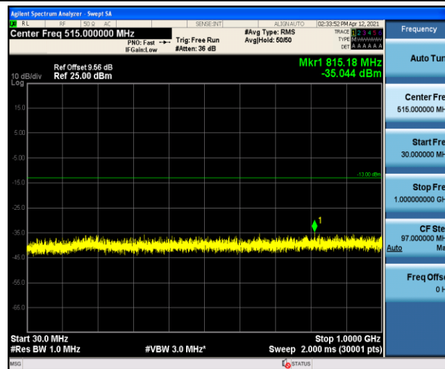
Band4-15MHz-16QAM-20325-1-0-High-30-1000
