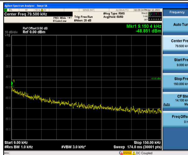
Band4-10MHz-16QAM-20175-1-0-Low-0.009-0.15
