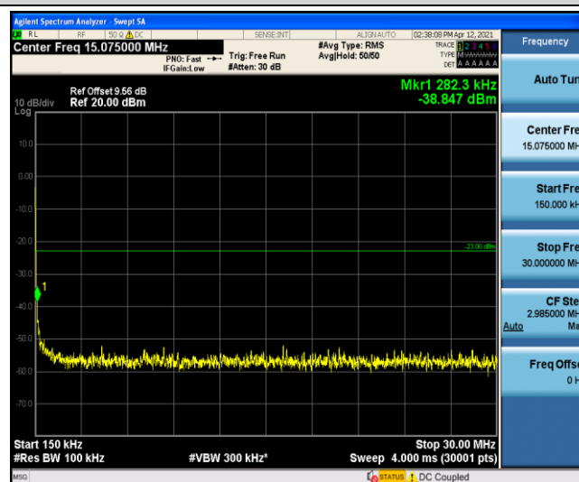
Band4-15MHz-16QAM-20175-1-0-Low-0.15-30
