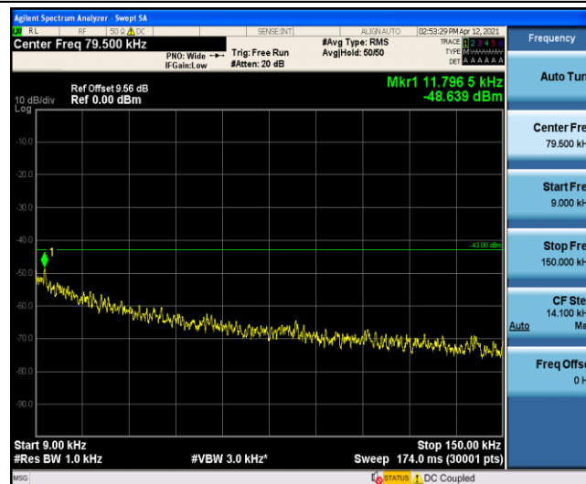
Band4-15MHz-QPSK-20025-1-0-Low-0.009-0.15
