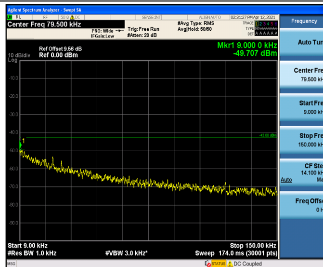
Band4-15MHz-QPSK-20325-1-0-High-0.009-0.15
