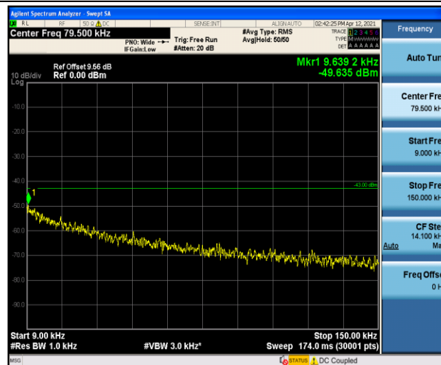
Band4-10MHz-16QAM-20000-1-0-Low-0.009-0.15
