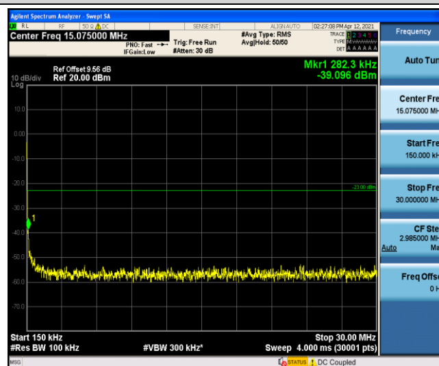
Band4-10MHz-QPSK-20175-1-0-Low-0.15-30
