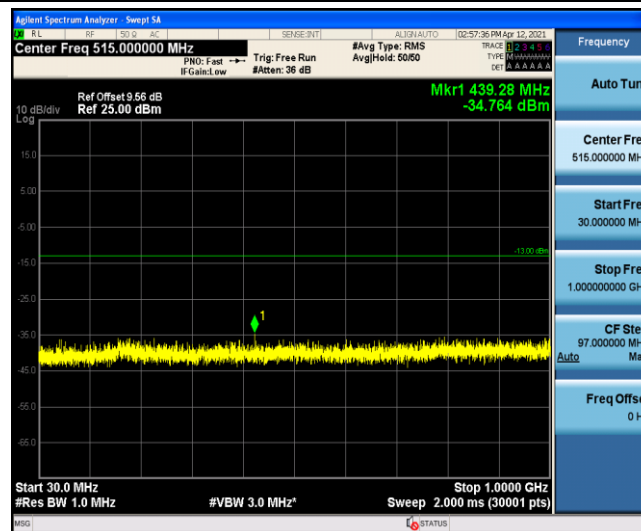
Band4-5MHz-QPSK-20175-1-0-Low-30-1000
