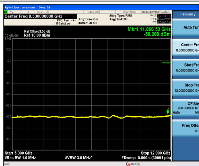
Band4-5MHz-16QAM-19975-1-0-Low-5000-12000
