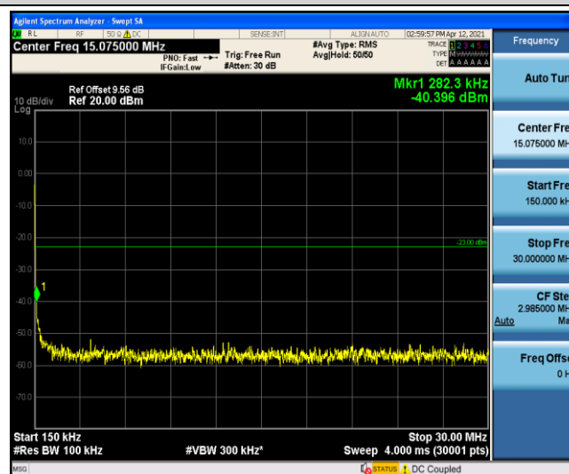
Band4-5MHz-16QAM-20175-1-0-Low-0.15-30
