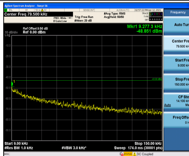
Band4-5MHz-QPSK-20175-1-0-Low-0.009-0.15
