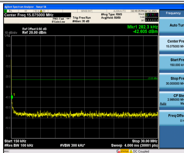
Band4-10MHz-QPSK-20350-1-0-High-0.15-30
