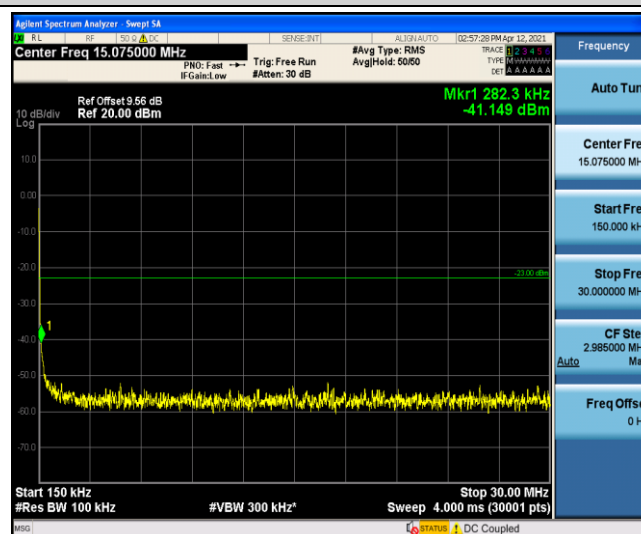
Band4-5MHz-QPSK-20175-1-0-Low-0.15-30
