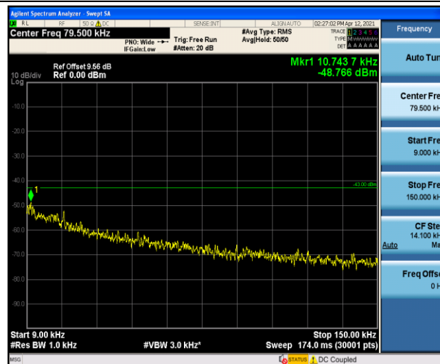
Band4-10MHz-QPSK-20175-1-0-Low-0.009-0.15
