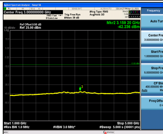
Band4-5MHz-QPSK-20375-1-0-High-1000-5000
