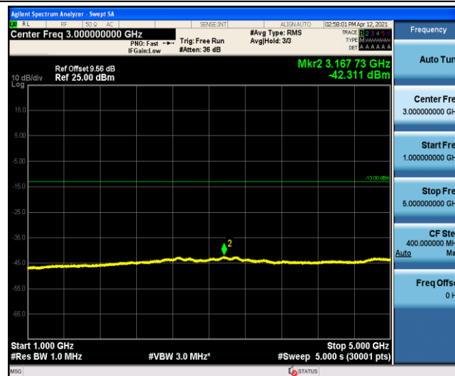
Band4-5MHz-QPSK-20175-1-0-Low-1000-5000
