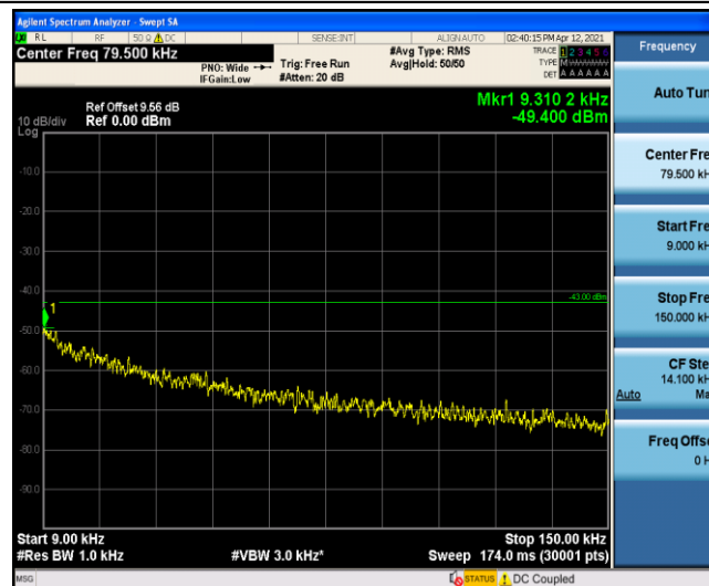
Band4-10MHz-QPSK-20000-1-0-Low-0.009-0.15
