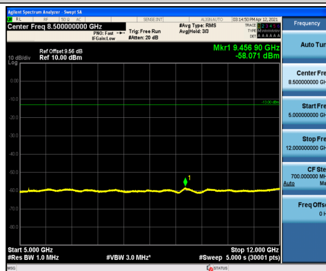
Band4-5MHz-QPSK-20375-1-0-High-5000-12000
