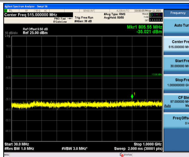
Band4-5MHz-16QAM-20175-1-0-Low-30-1000
