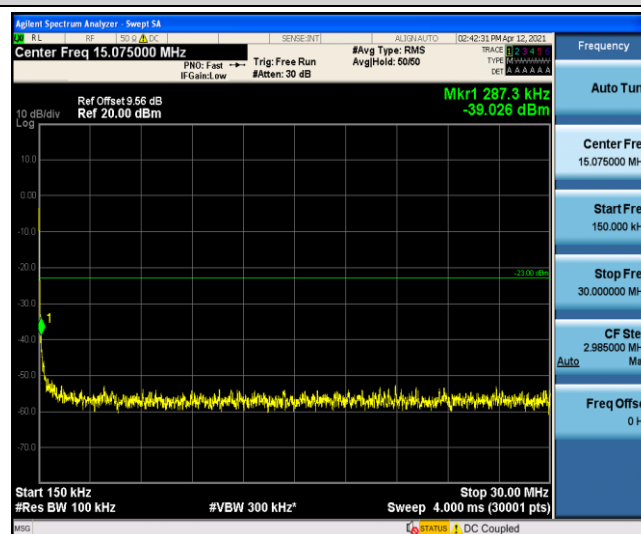
Band4-10MHz-16QAM-20000-1-0-Low-0.15-30
