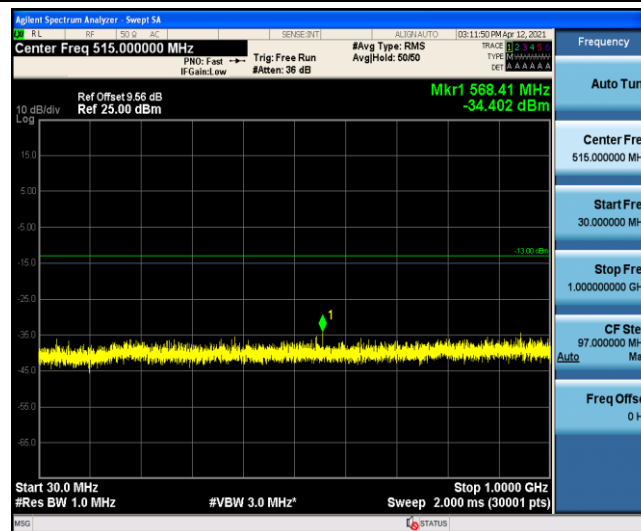
Band4-5MHz-16QAM-19975-1-0-Low-30-1000
