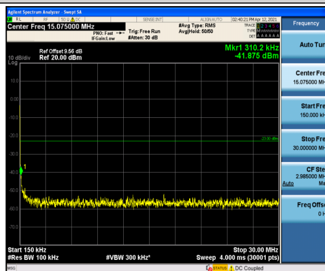
Band4-10MHz-QPSK-20000-1-0-Low-0.15-30
