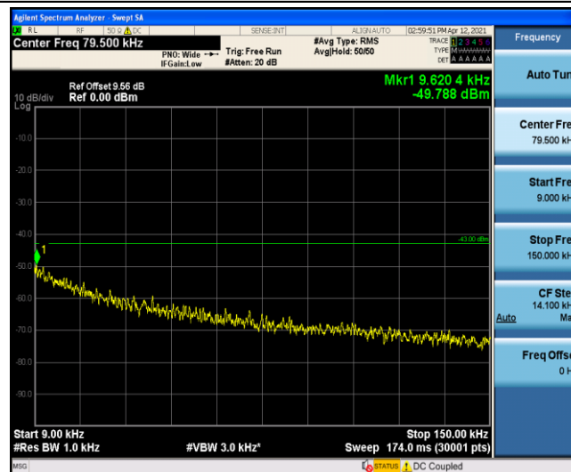
Band4-5MHz-16QAM-20175-1-0-Low-0.009-0.15
