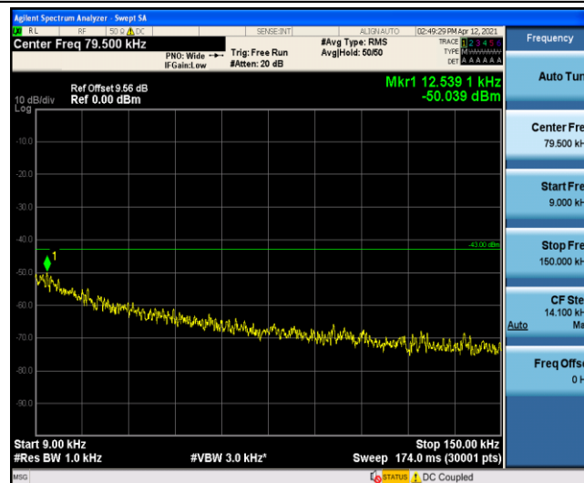
Band4-10MHz-QPSK-20350-1-0-High-0.009-0.15
