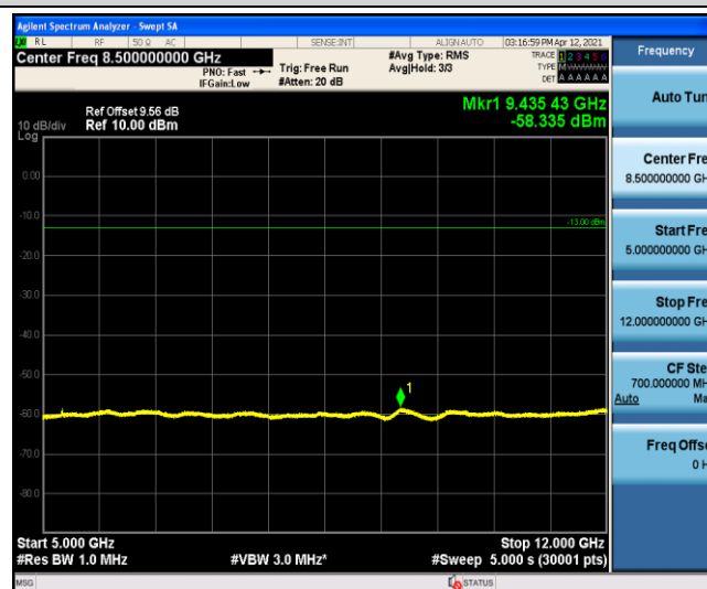
Band4-5MHz-16QAM-20375-1-0-High-5000-12000
