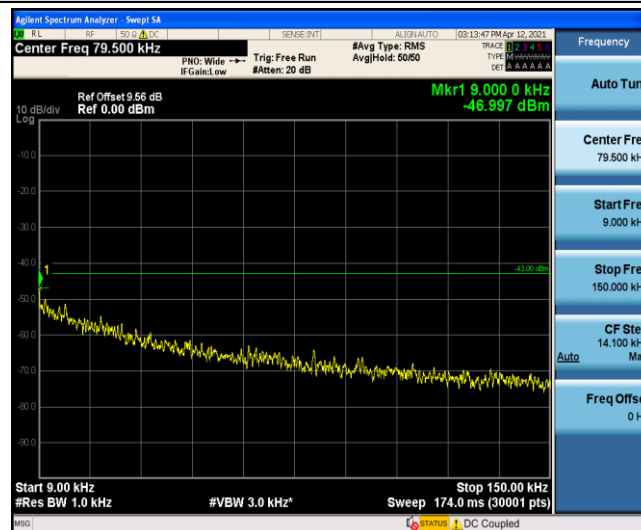
Band4-5MHz-QPSK-20375-1-0-High-0.009-0.15
