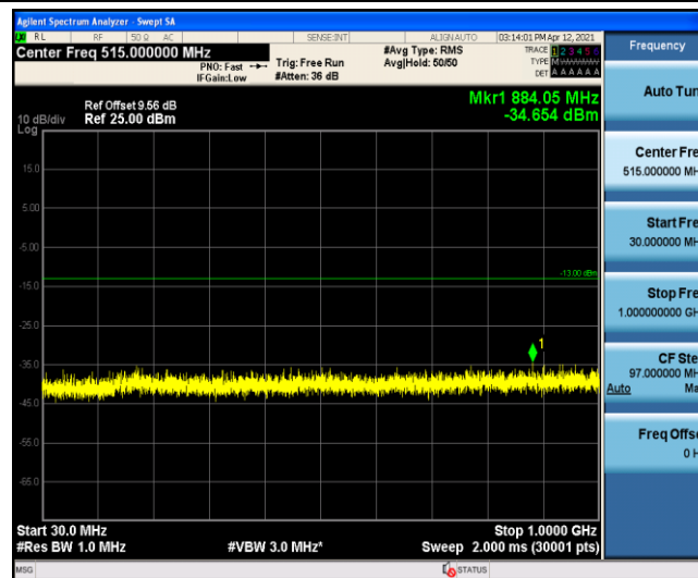
Band4-5MHz-QPSK-20375-1-0-High-30-1000
