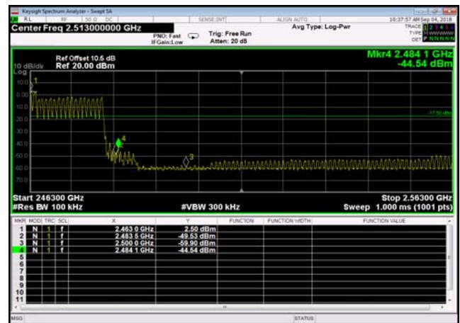
Conducted Emission: pi/4DQPSK,2480,2DH5 ,Band Edge
