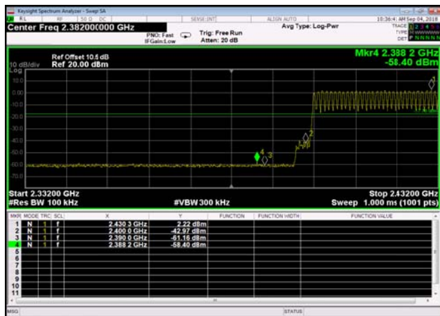
Conducted Emission: pi/4DQPSK,2402,2DH5 ,Band Edge
