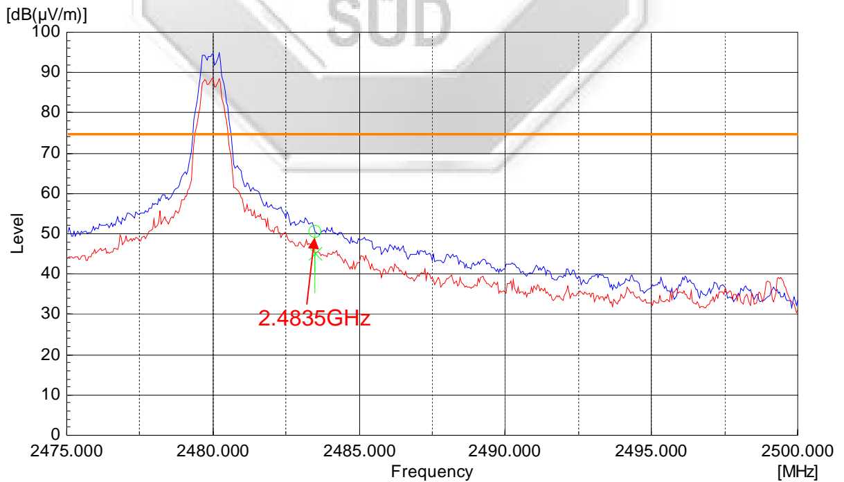
Plot 39 – Upper Band Edge at 2.4835GHz
