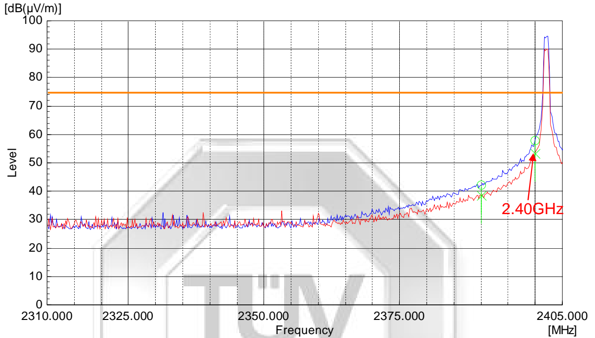
Plot 38 – Lower Band Edge at 2.4000GHz
