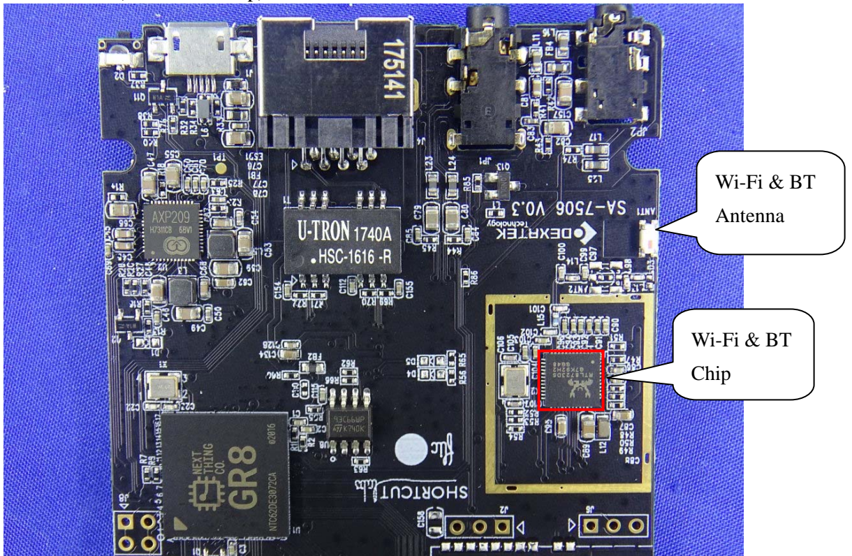
(10) EUT Photo – (WiFi + BT Chip)
