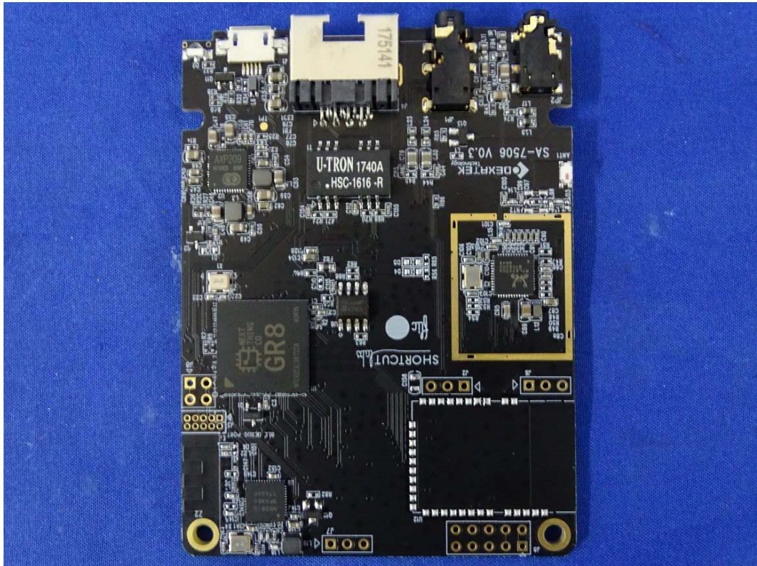
(10) EUT Photo – (WiFi + BT Chip)
