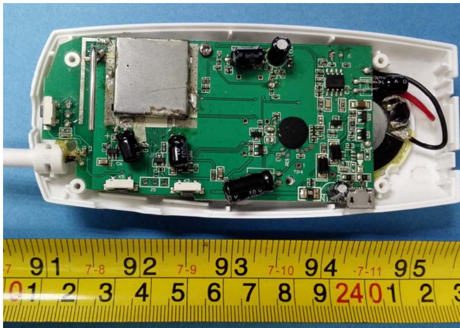
EUT –RF Chip View
