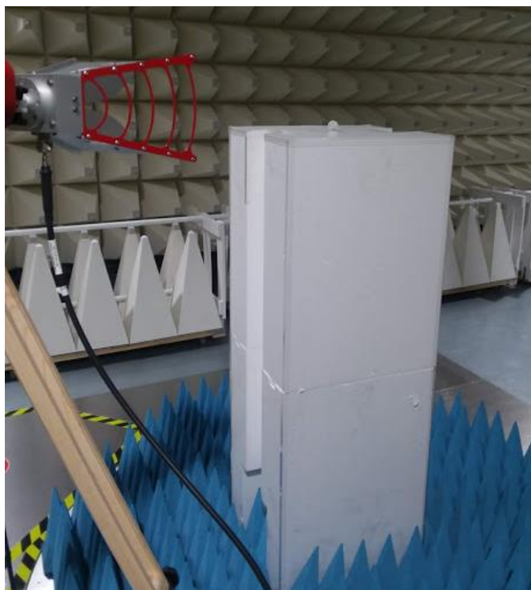
Figure C2: Radiated Emission measurement setup for frequencies above 1GHz
