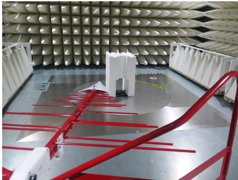
Figure C1: Radiated Emission measurement setup for frequencies below 1GHz
