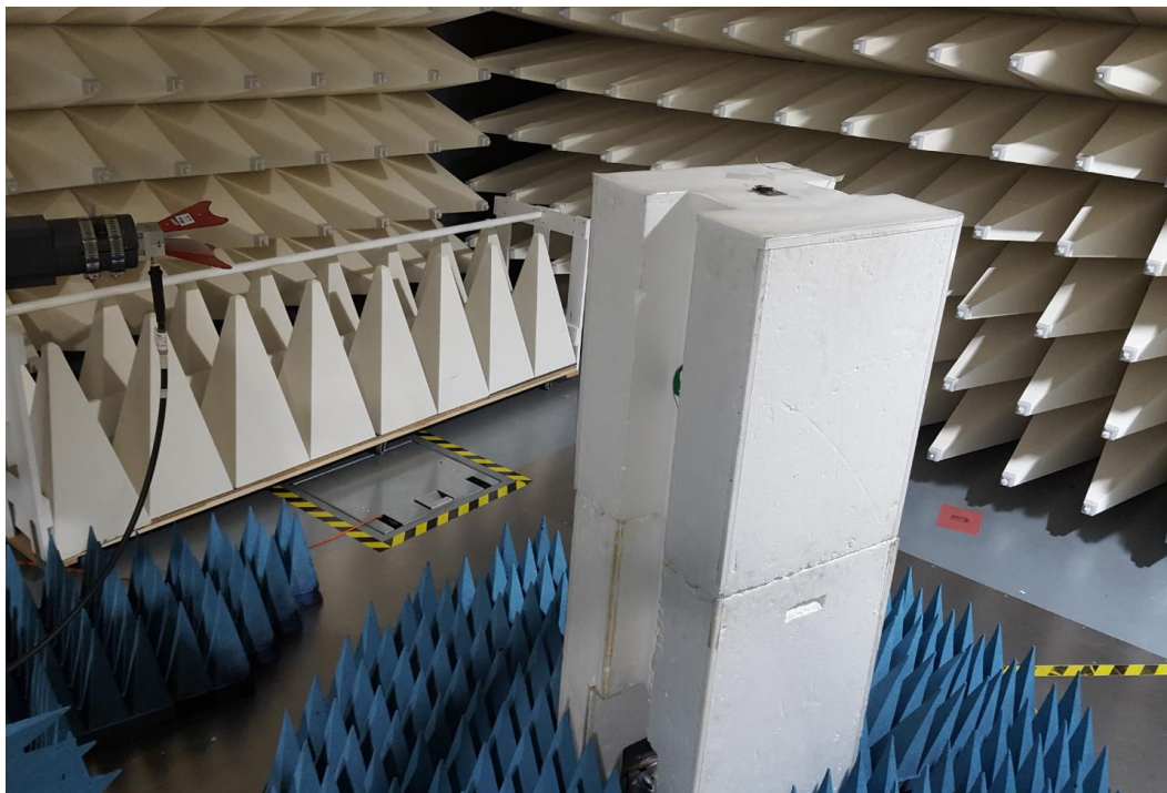
Figure B6. High Range Radiated Emission test setup 18-26 GHz
