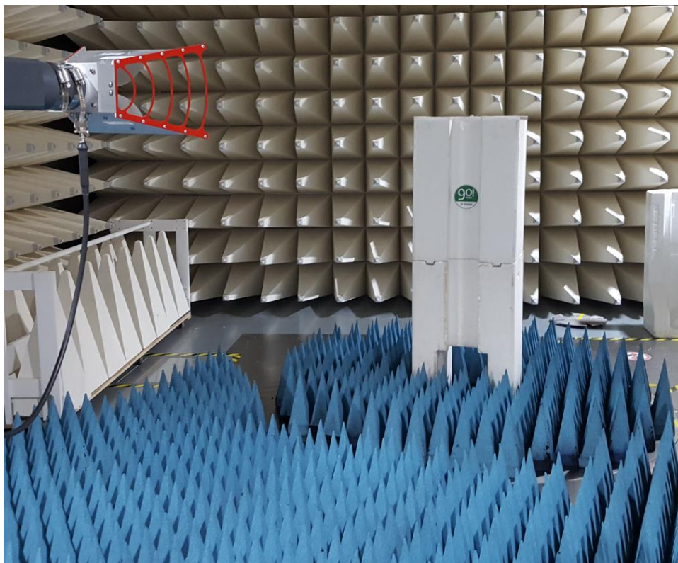
Figure B5. High Range Radiated Emission test setup 1-18GHz
