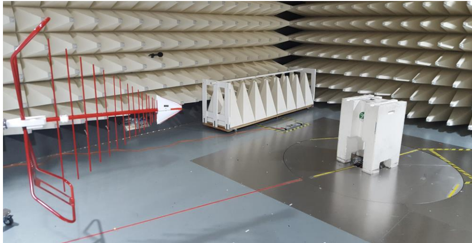
Figure B4. Low Range Radiated Emission test setup
