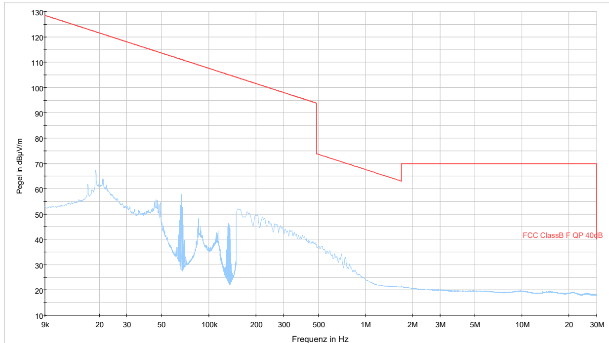
Preview Result 2-AVG Preview Result 1-QPK FCC ClassB F QP 40dB Final_Result QPK Final_Result AVG
