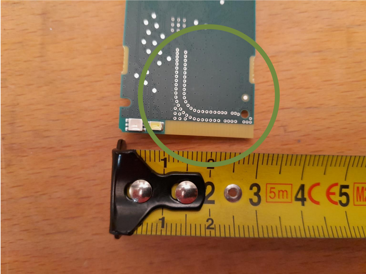
Bottom view of the PCB:
