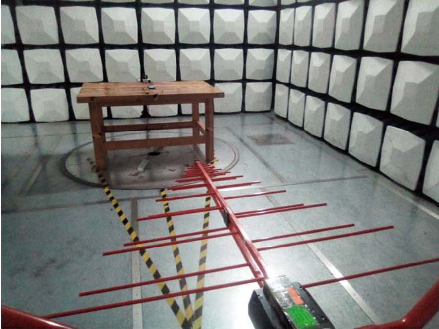
Radiated Emission Below 1GHz View (Adapter #2)
