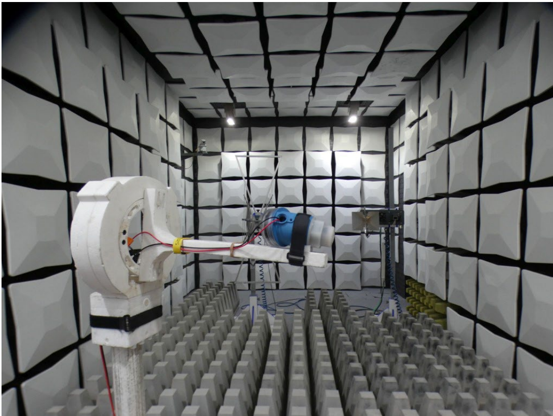
Photo 5: Test setup for radiated measurements above 18 GHz
