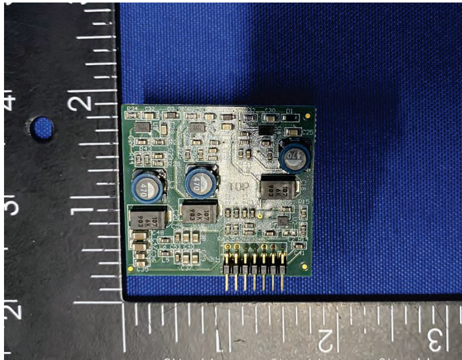
(11) EUT Photo
