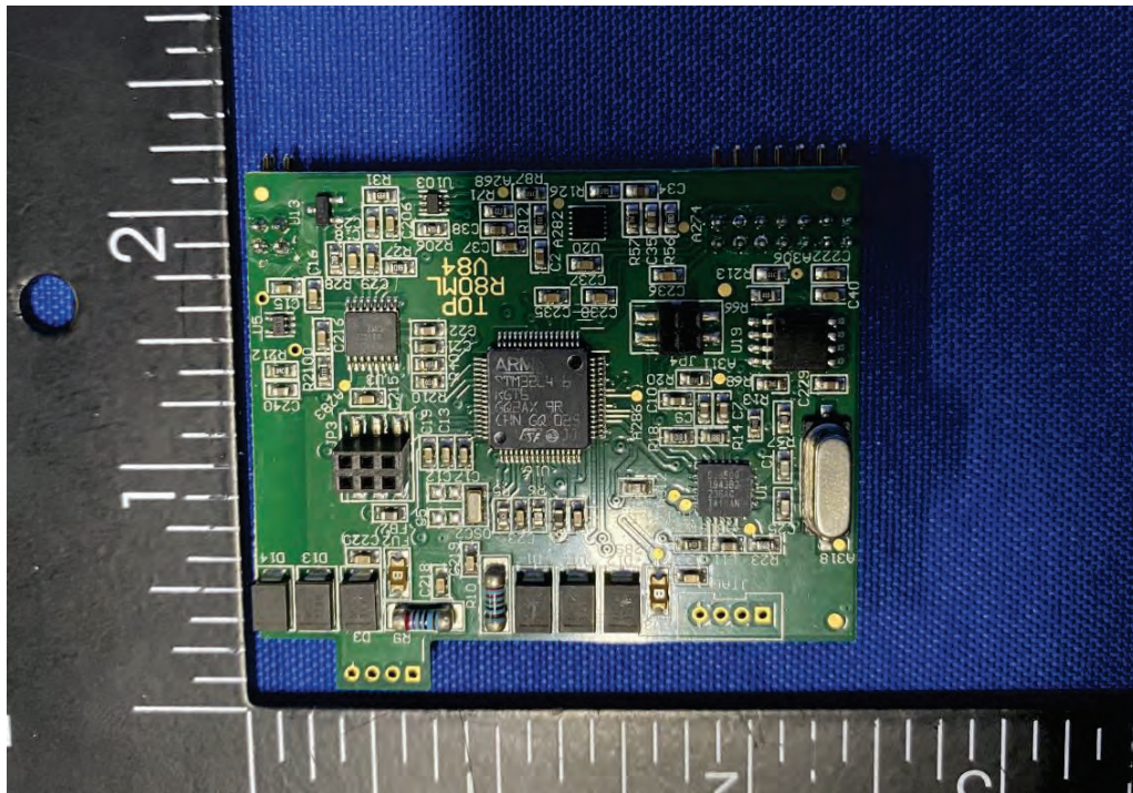
(7) EUT Photo
