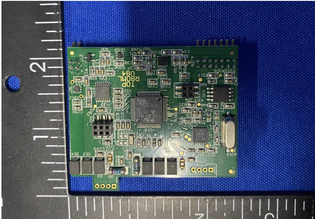
(7) EUT Photo
