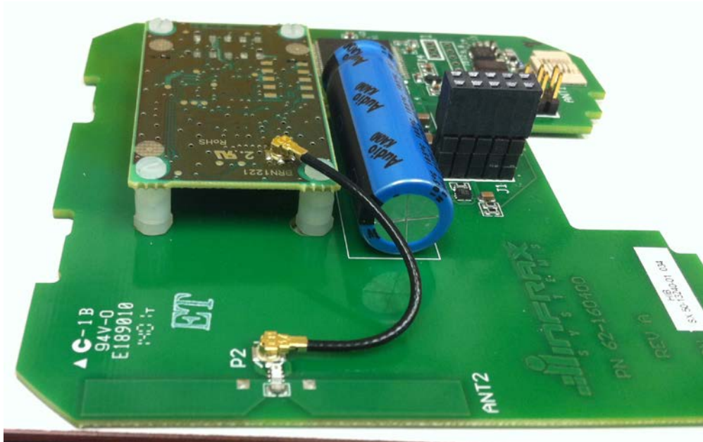
Figure 4: EUT with Antenna – View 2
