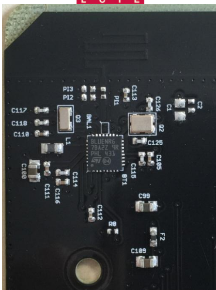
RF Circuitry
