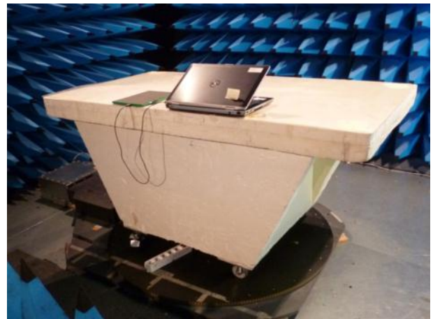
Test setup in anechoic chamber (USB mode):
