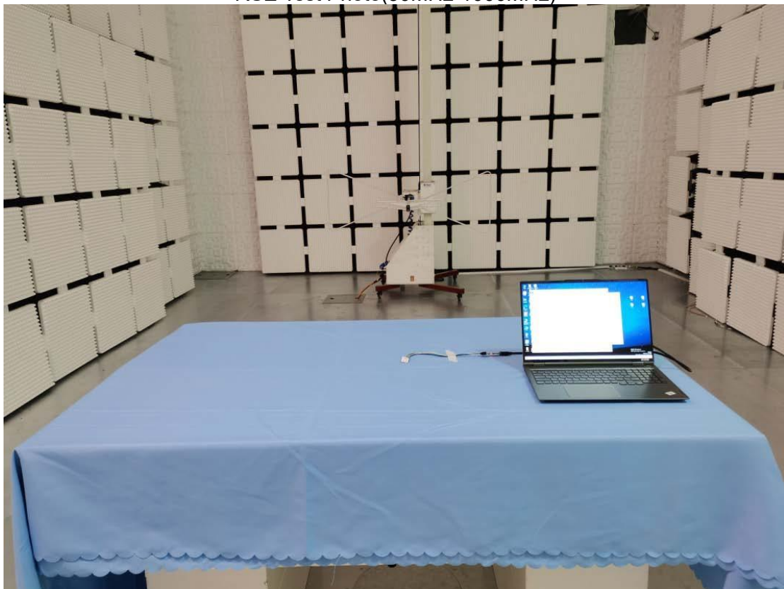
RSE Test Photo(30MHz-1000MHz)
